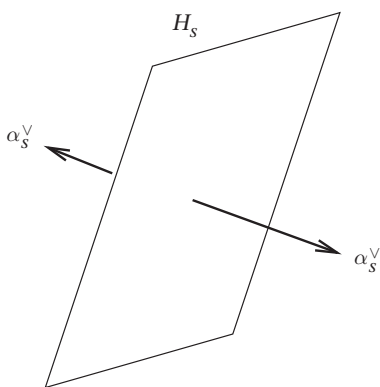
Figure 5. (a) \sigma_s negates \alpha_s^v and fixes H_s .
