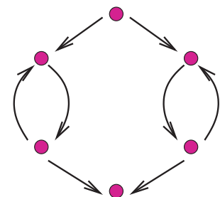
(b) \Gamma_L
