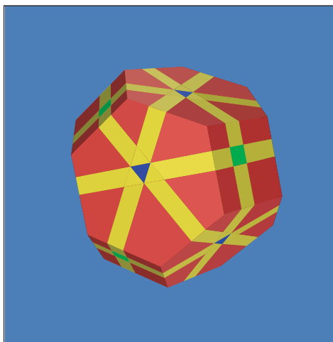
Figure 9. Two views of the cells of \tilde{A}_3 . (a)
