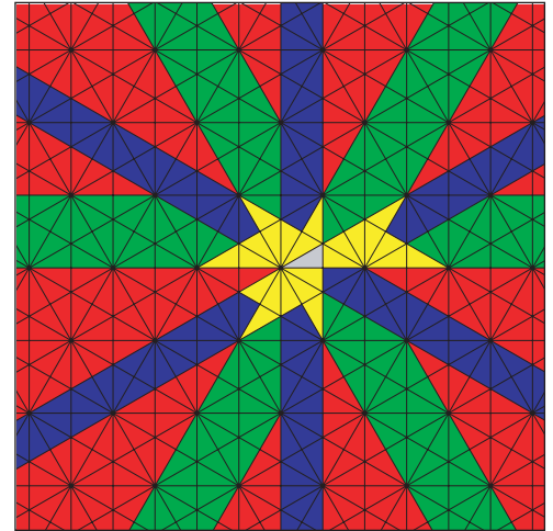
Figure 3. \tilde{G}_2 = W_{236} .
