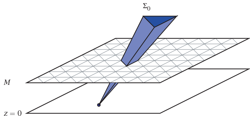
(b) Slicing the Tits cone for \tilde{A}_2 .
