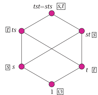
(a) \mathfrak{S}_3
