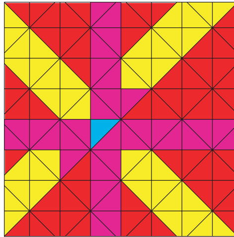
Figure 11. (a) \tilde{C}_2
