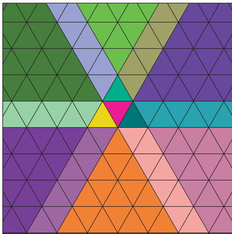
Figure 8. (a) \tilde{A}_2 sign-type regions.
