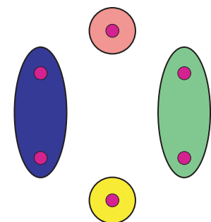
(c) Left cells
