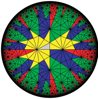
Figure 4. (a) W_{237}
