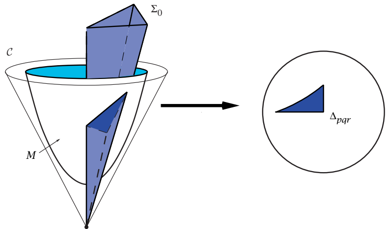
Figure 6. Slicing the Tits cone for a hyperbolic triangle group.
