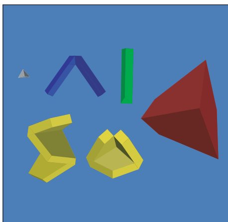
Figure 10. \tilde{A}_3 left cells up to congruence.
