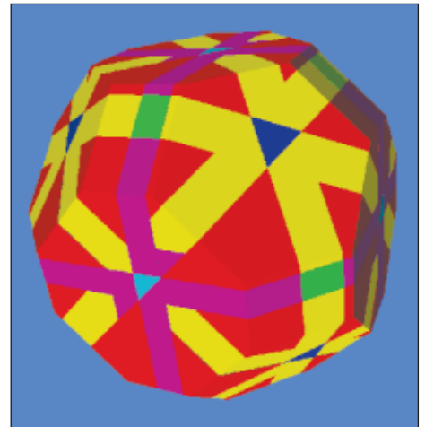
(b) \tilde{C}_3
