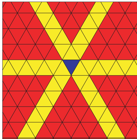
(b) \tilde{A}_2 cells.
